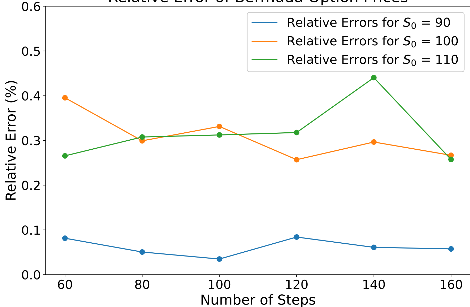
Relative Error of Bermuda Option Prices
